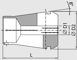
Spannzange Power Collet/Power Collet
